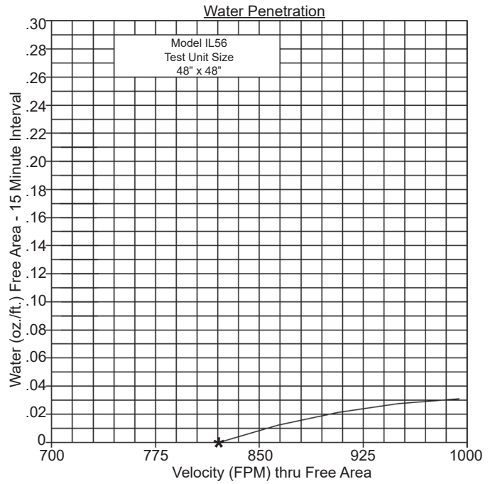
821 (FPM) Beginning Point of Water Penetration.
